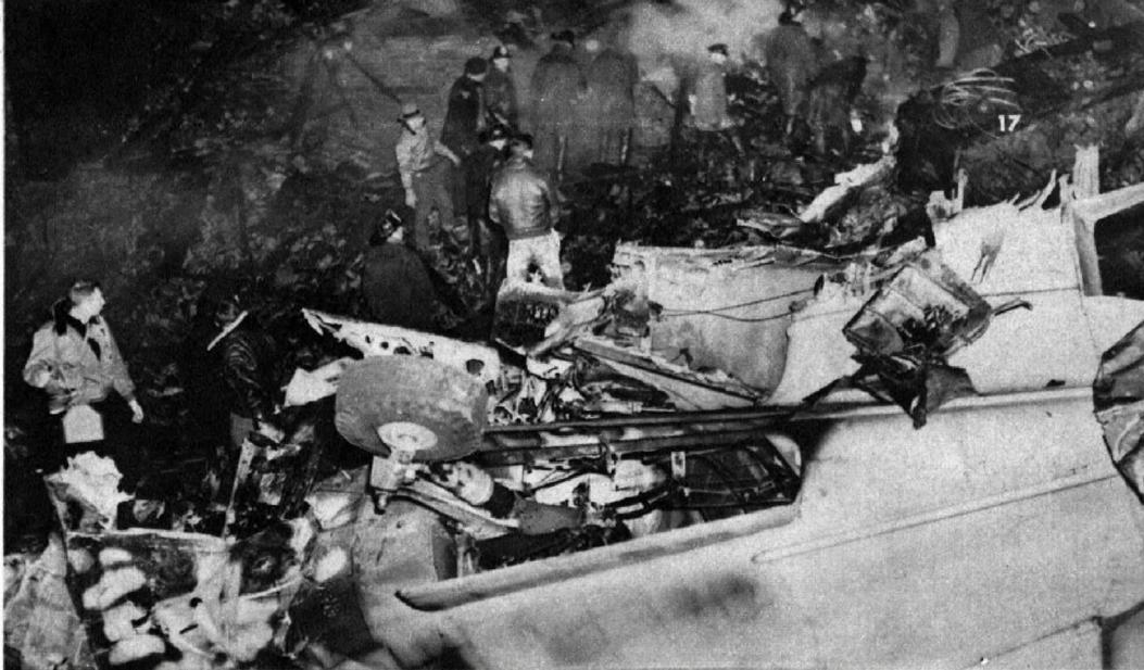
Crash No. 1 in Elizabeth took the lives of all 56 aboard the Miami-bound plane, but only one person on ground was hurt. The cause was failure of bolt assemblies to anchor a cylinder
