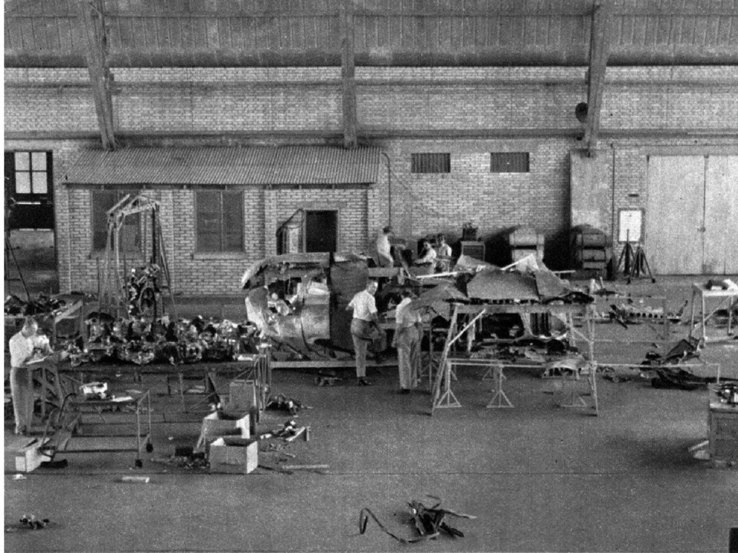
Temporary laboratories, like this one in Egypt, are set up wherever an American craft crashes, for examination of all remaining plane parts. When cause is found, safety measures follow
